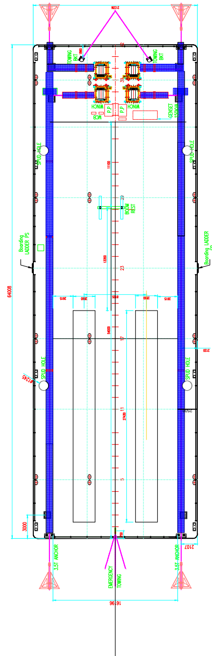
MAIN DECK
